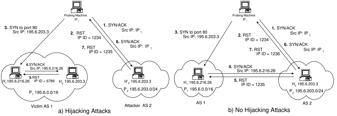
Fig. 6. Reflect-scan: detection of hijacking subnet of a prefix (type-3 and type-4 attacks).
