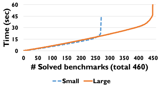
Figure 25. FIDEX with different token sets (114 v.s. 46).
