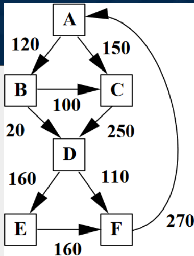
Figure 1. Example in which edge profiling does not identify the most frequently executed paths. The table contains two different path profiles. Both path profiles induce the same edge execution frequencies, shown by the edge frequencies in the control-flow graph. In path profile Prof1 , path ABCDEF is most frequently executed, although the heuristic of following edges with the highest frequency identifies path ACDEF as the most frequent.
