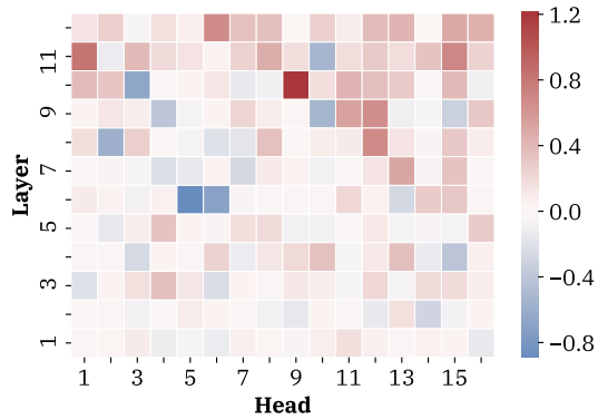
(a) XSum
