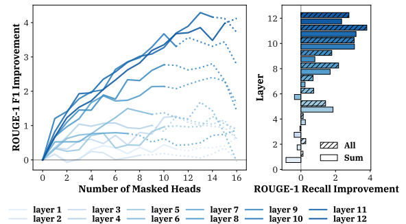
(a) XSum
