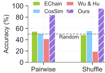
Figure 4: Accuracy of our coherence model compared to different baselines and Wu and Hu (2018) on PAIRWISE and SHUFFLE test sets.
