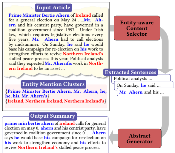
Figure 2: Our proposed entity-driven abstractive summarization framework. Entity-aware content selector extracts salient sentences and abstract generator produces informative and coherent summaries. Both components are connected using reinforcement learning.
