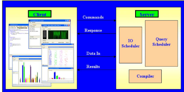
Figure 1. SMM Architecture
