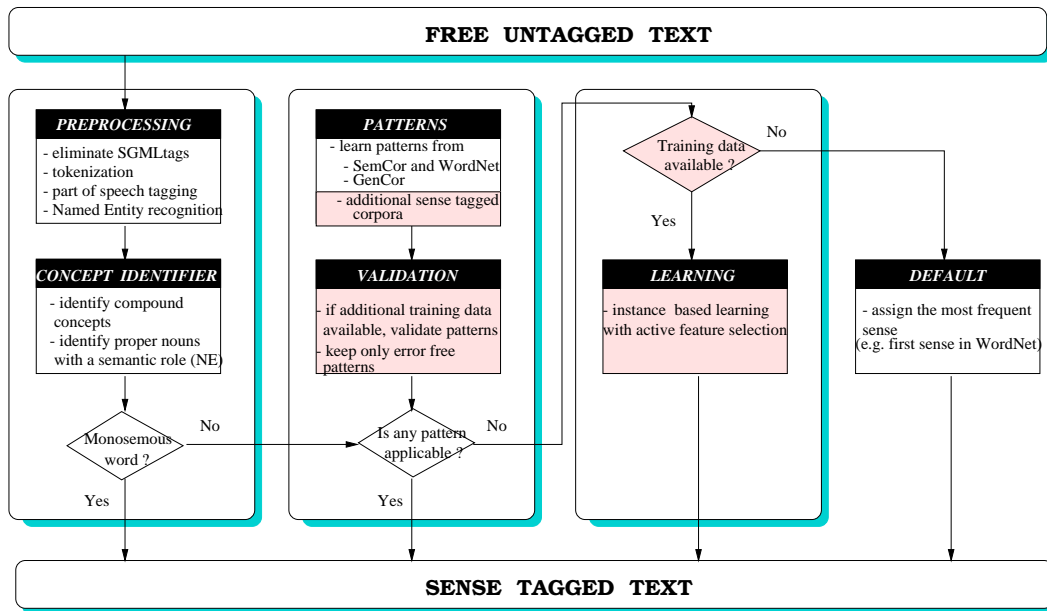
Fig. 1. System architecture
