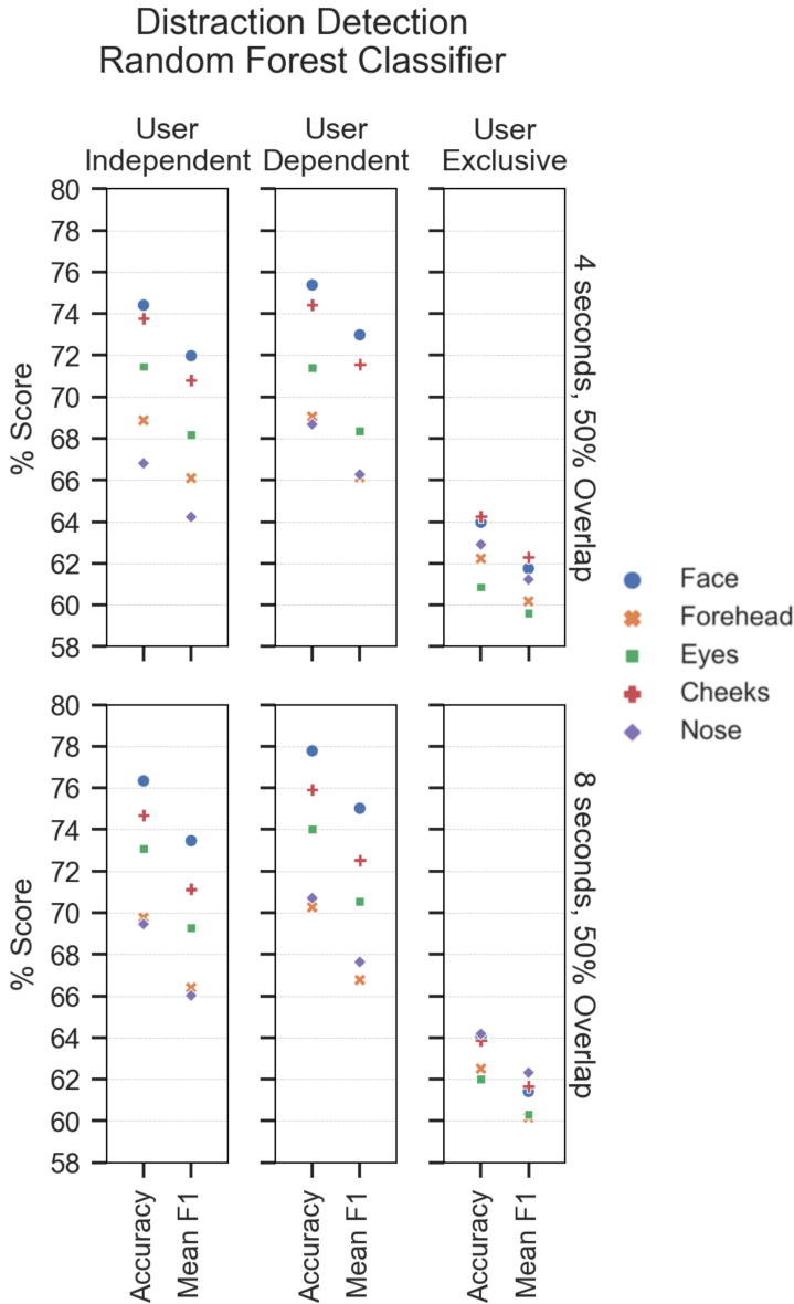
Fig. 14. Performance metrics on distracted VS non-distracted driving classification for each ROI in the Thermal modality.
