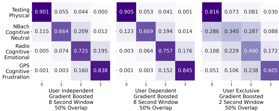
Fig. 12. Confusion matrices on distraction recognition as a 4-class problem for the best results of Table 9 for each modeling approach
