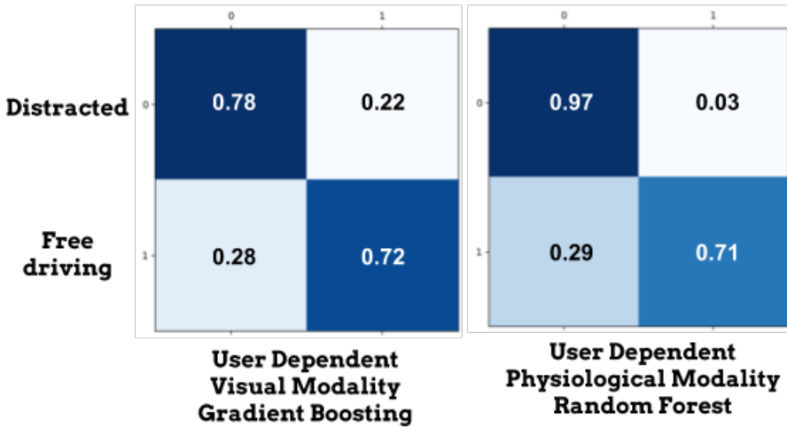
Fig. 4. Confusion matrices on distracted VS non-distracted driving classification for the best results of Table 2
