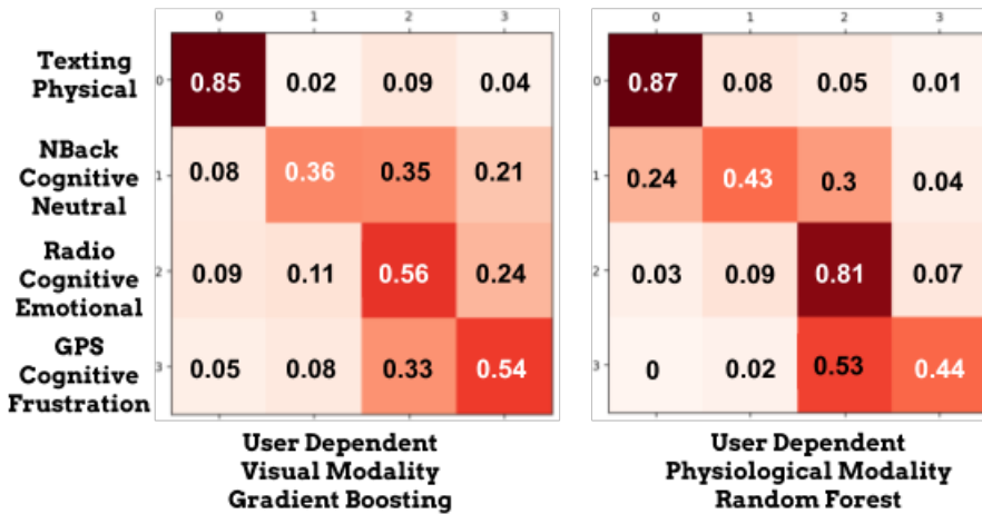
Fig. 6. Confusion matrices on distraction recognition as a 4-class problem for the best results of Table 4
