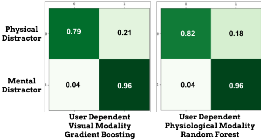
Fig. 5. Confusion matrices on distraction recognition as a 2-class problem for the best results of Table 3
