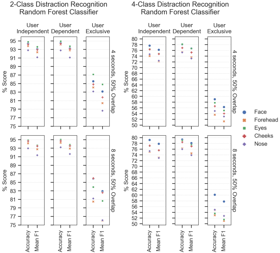
Fig. 15. Performance metrics on distraction recognition for each ROI in the Thermal modality for each modeling approach.
