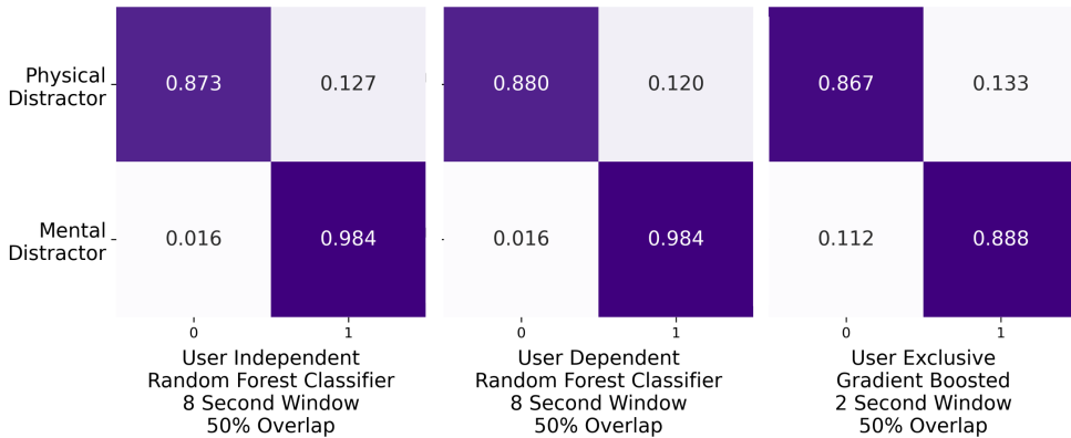
Fig. 11. Confusion matrices on distraction recognition as a 2-class problem for the best results of Table 8 for each modeling approach
