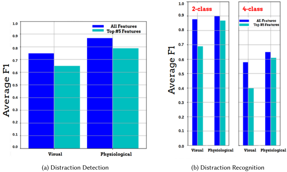
Fig. 9. Performance comparison between best models (User-Dependent scheme) trained on the top 5 features of each modality VS all the available features.
