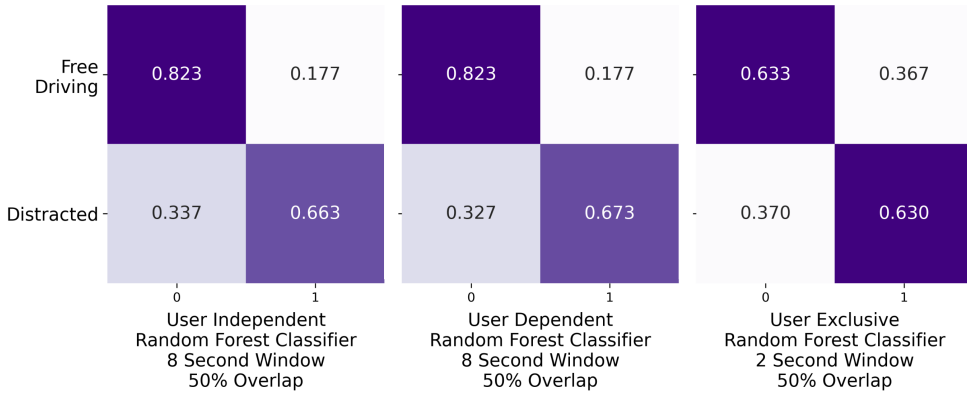
Fig. 10. Confusion matrices on distracted VS non-distracted driving classification for the best results of Table 7 for each modeling approach.
