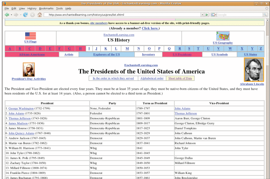
Figure 1. Typical use of the table tag to describe relational data that has structure never explicitly declared by the author, including metadata consisting of several typed and labeled columns, but that is obvious to human observers. The navigation bars at the top of the page are also implemented through the table tag but do not contain relational-style data.
