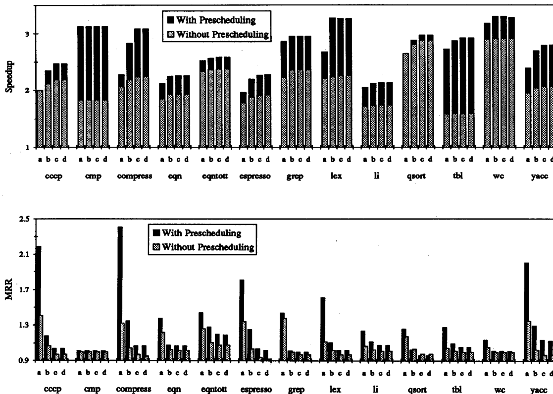
Fig. 6. The performance of prescheduling for processors with various register file sizes. Processors a, b, c, and d have 24, 32, 48, and 64 registers, respectively. All the processors, except the base architecture, have issue rate 4 and support the general percolation model. The base architecture is a single-issue processor with no prescheduling, restricted percolation, and 32 registers.
