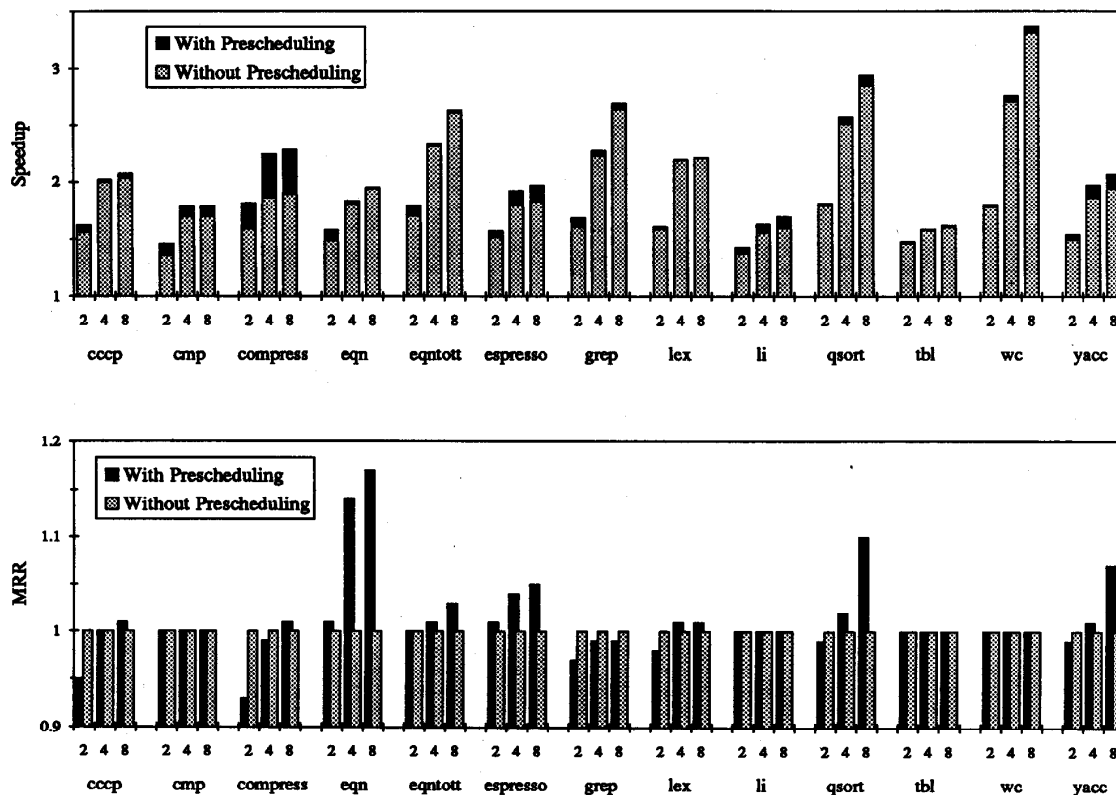
Fig. 2. The performance of prescheduling for the superscalar versions of existing architectures. The base architecture is the single-issue processor with no prescheduling. All the processors have 32 registers.
