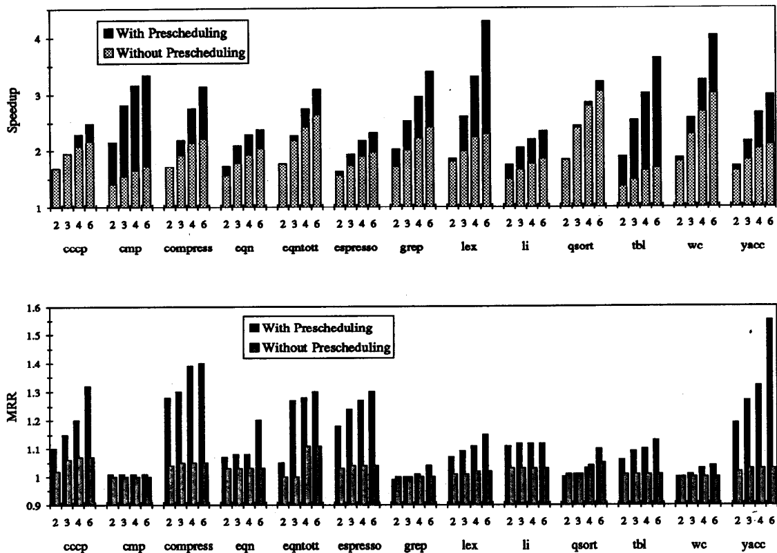
Fig. 5. The performance of prescheduling for the superpipelined versions of architectures that support general percolation. The base architecture is a single-issue processor with no prescheduling and restricted percolation. 2 and 3 are single-issue, 2X- and 3X-superpipelined processors, respectively. 4 and 6 are dual-issue, 2X- and 3X-superpipelined processors, respectively. All the processors have 32 registers.
