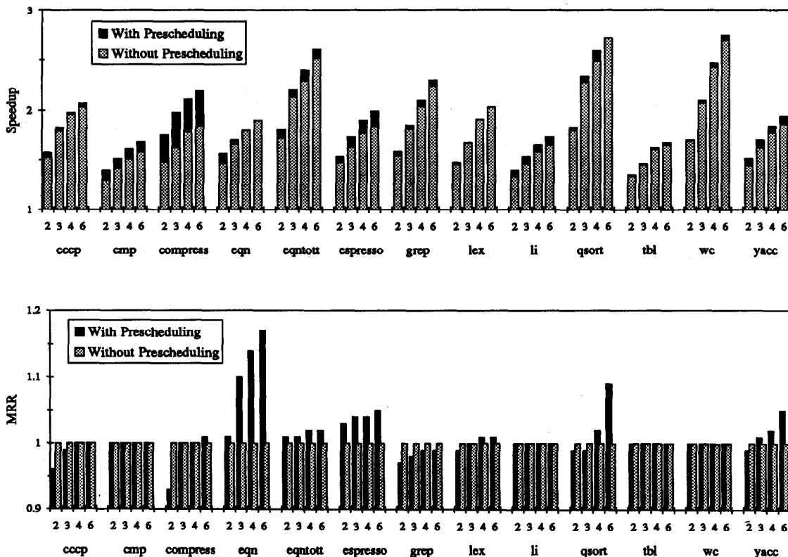
Fig. 3. The performance of prescheduling for the superpipelined versions of existing architectures. The base architecture is the single-issue processor with no prescheduling. 2 and 3 are single-issue, 2X- and 3X-superpipelined processors, respectively. 4 and 6 are dual-issue, 2X- and 3X-superpipelined processors, respectively. All the processors have 32 registers.
