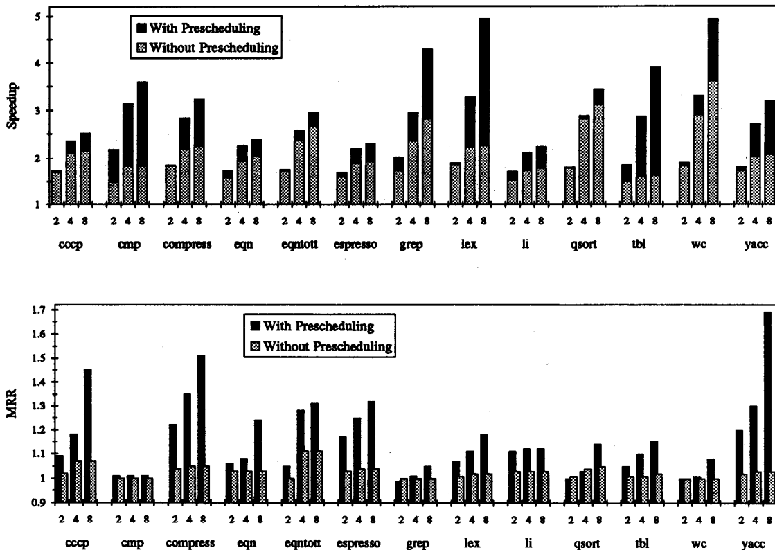
Fig. 4. The performance of prescheduling for the superscalar versions of architectures that support general percolation. The base architecture is a single-issue processor with no prescheduling and restricted percolation. All the processors have 32 registers.
