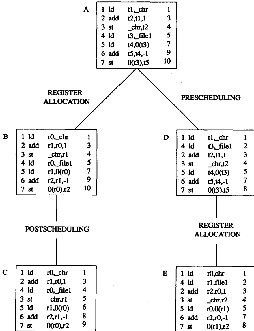
Fig. 1. Examples of postpass and prepass code scheduling.
