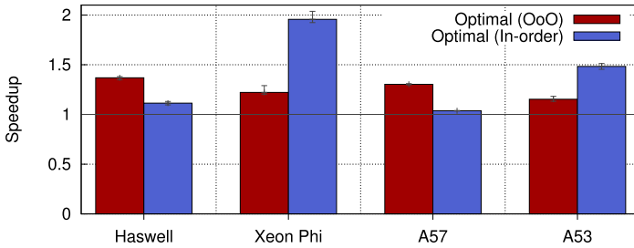
(a) Graph500 -s16 -e10
