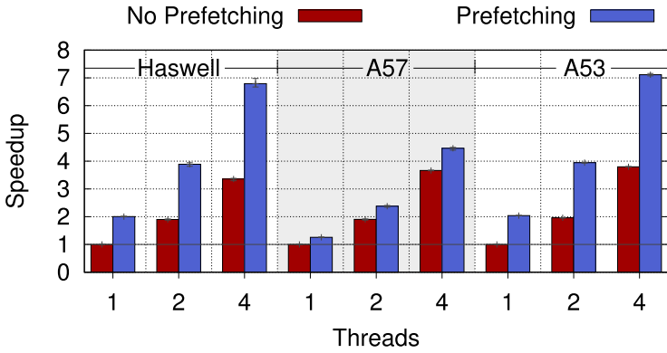
(a) Parallel HJ-2, using pthreads.
