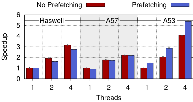
(b) Parallel CG, using OpenMP.
