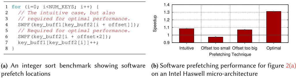
Fig. 2. Inserting software prefetches for maximal performance is a challenge even in simple cases. In (a), the intuitive prefetch to insert is only at line 4, whereas optimal performance also requires that at line 6. In (b), intuitive schemes leave performance on the table, and choosing the correct offset is critical for high performance.
