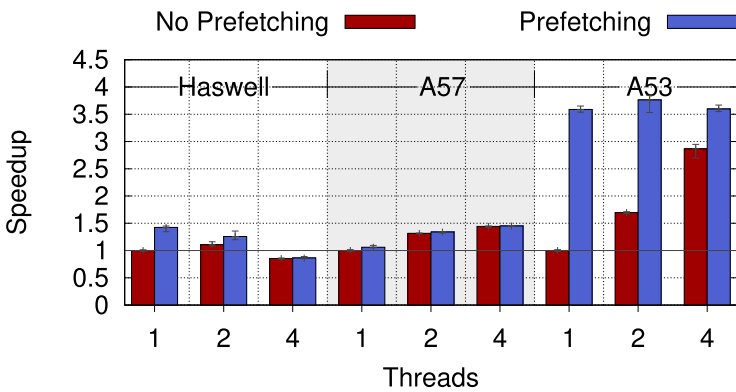
(c) Parallel IS, using OpenMP.
