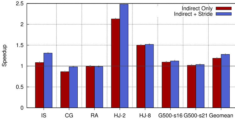
Fig. 5. Performance of inserting staggered stride software prefetches along with the indirect prefetch, compared to the indirect alone, for Haswell, with our automated scheme.
