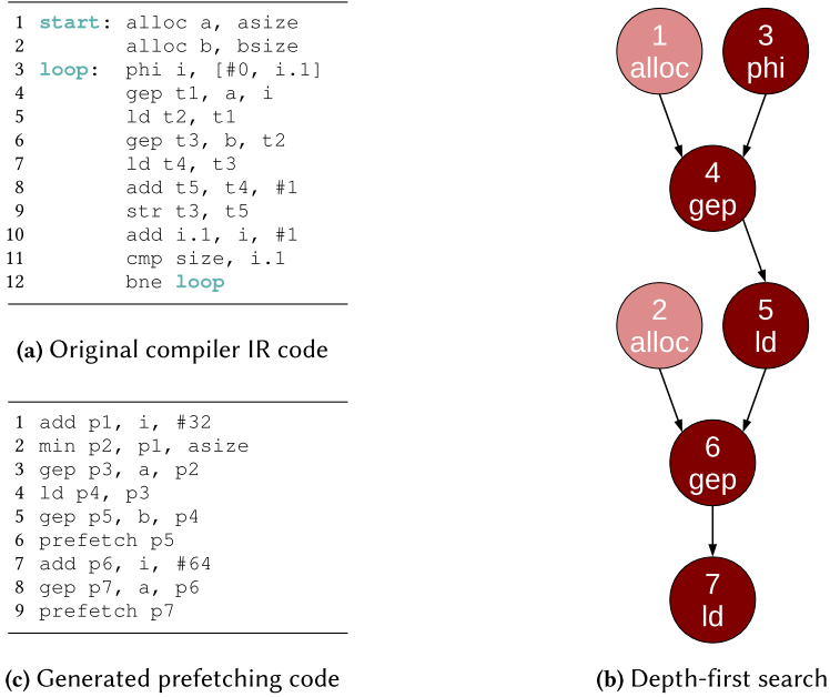
Fig. 3. Our pass running on an integer sort benchmark.
