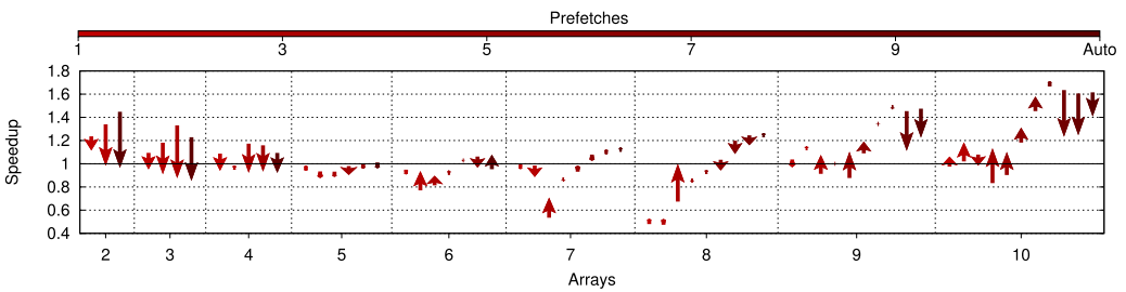
Fig. 17. Performance of Kangaroo for Haswell, with look-ahead constant ( c ) set to 16 compared with the default 64. For arrows pointing downward, the smaller look-ahead reduces performance.
