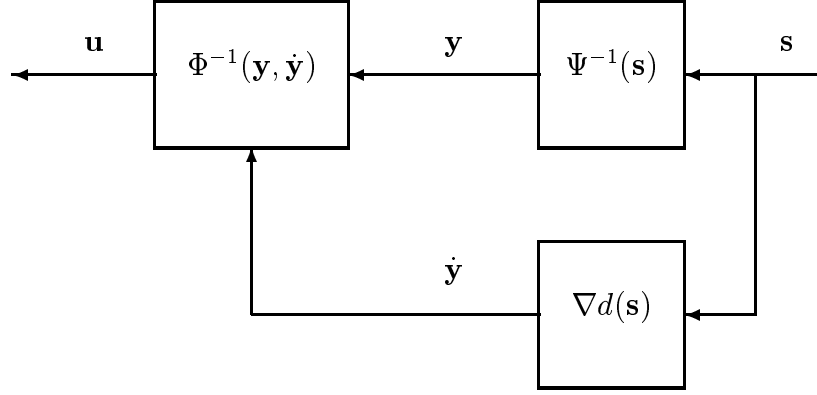
Figure 6: One of many ways to realize the control law \mathbf{u} = \chi_i(\mathbf{s}) in Figure 5, in case there is an observer \Psi^{-1}(\mathbf{s}) that describes the local environment in terms of a local state vector \mathbf{y} , the control law can be described as hill-climbing a distinctiveness measure d(\mathbf{s}) , and there is a pseudo-inverse \Phi^{-1}(\mathbf{y}, \dot{\mathbf{y}}) that determines \mathbf{u} .
