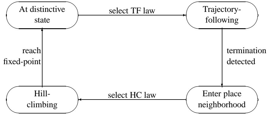
Figure 3: Distinctive places found by alternating trajectory-following and hill-climbing control laws.
