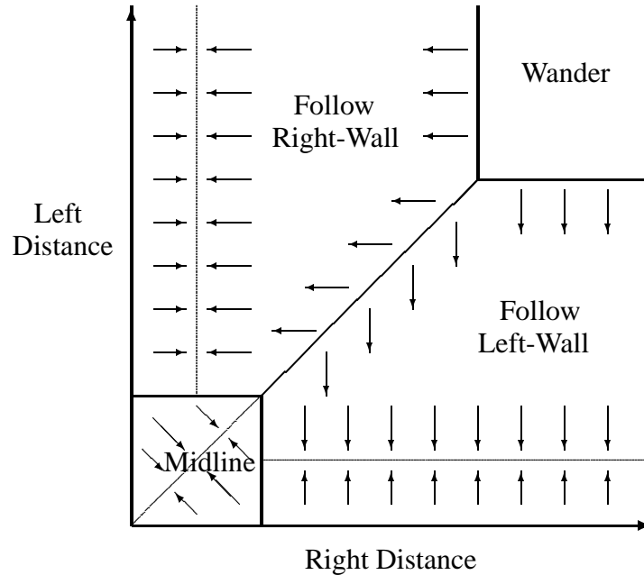
Figure 11: Selection criteria for trajectory-following control laws. In an office environment with range-sensors, a trajectory-following control law is selected depending on distances to obstacles on the left and on the right. Arrows show the direction of flow in the region appropriate to each control law.
