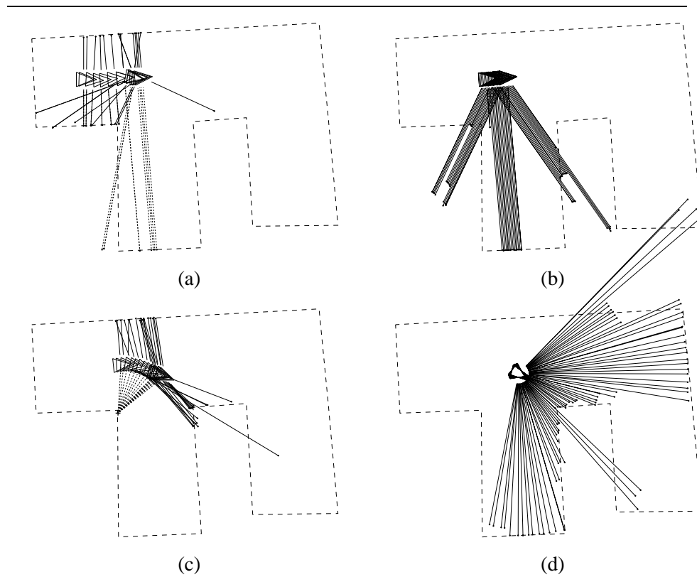
Figure 9: Control behaviors leading Spot (RWI B12) to a distinctive state. (a) Spot is following the midline when it detects sudden increase in distance to right wall. (b) Moving slowly, Spot localizes the convex corner in a local frame of reference. (c) Using “virtual sensing” of the convex corner, Spot follows a parabolic trajectory equidistant from corner and wall, until reaching a point the same distance from the forward obstacle. (d) Spot rotates to face directly towards the forward obstacle, defining the distinctive state.
