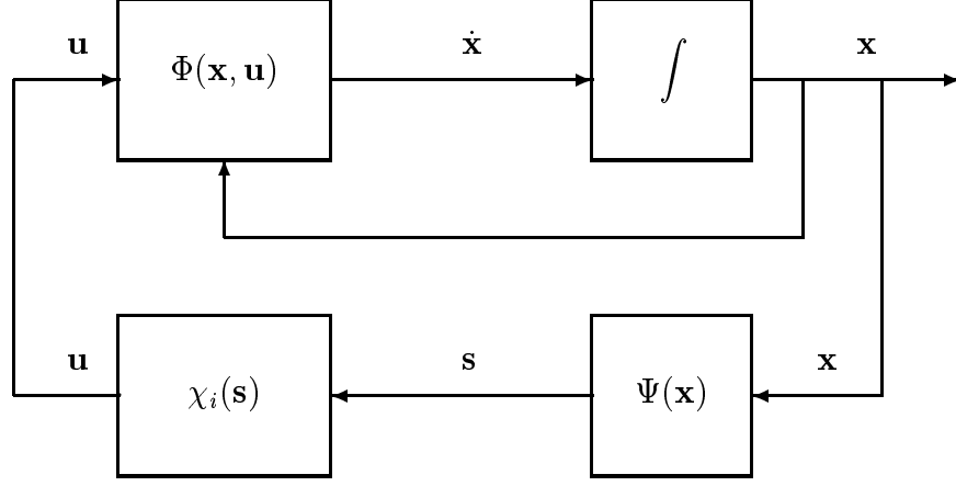
Figure 5: Within any given qualitatively uniform segment of the environment, the robot behaves according to a block diagram representing equations (1), (2) and (3) in section 2.1. The selection of the control law \chi_i is the external input that determines the robot's behavior.
