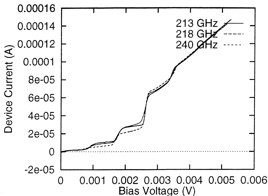
FIGURE III Pumped I-V Curves at 213, 218, 240 GHz with Suppressed Josephson Effect
