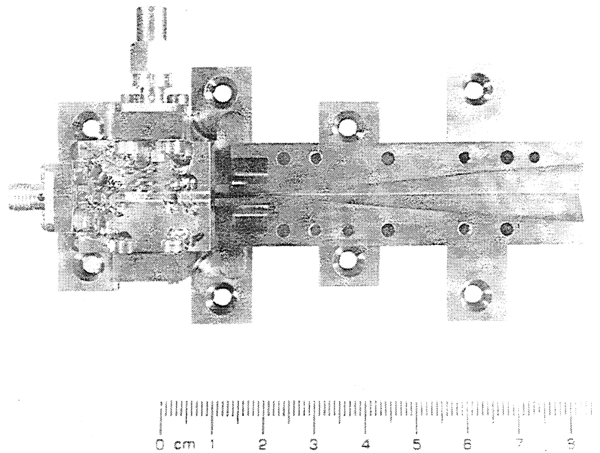
FIGURE II A Photograph of the Mixer Block Lower Half and the IF-bias board
