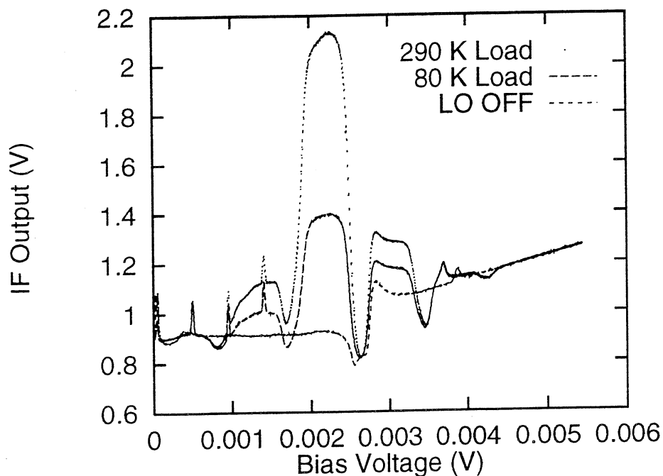
FIGURE IV Responses of the IF output of the Mixer to Hot (290 K) and Cold (80 K) Loads at 213 GHz
