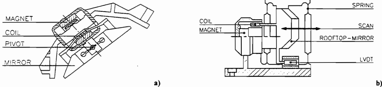
Figure 4. Drawing showing the HIFI mechanisms: a) chopper; b) diplexer
