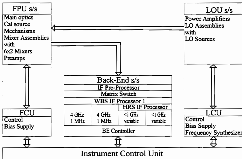
Figure 1. Block diagram of the HIFI instrument
