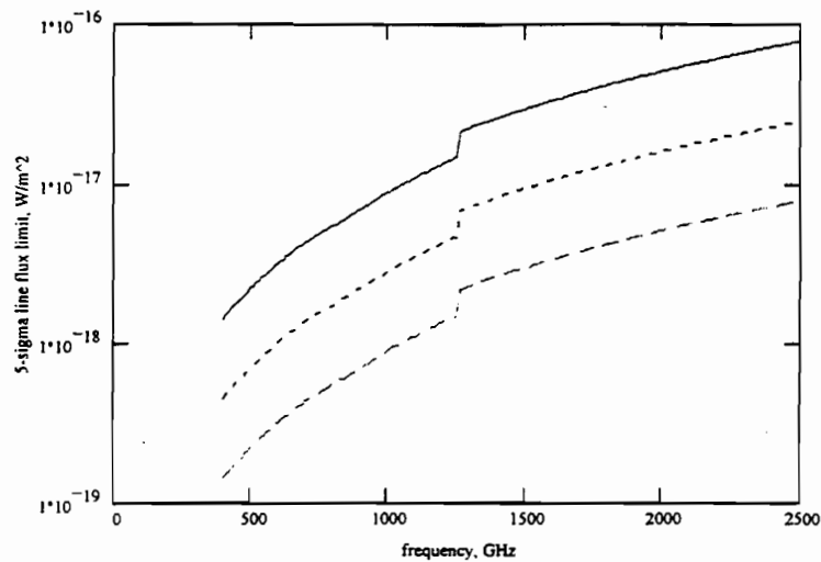
Figure 8. 5-sigma point-source line flux detection limits for a 1 hour integration and for three velocity resolutions starting from the top: 300, 30, and 3 km/s
