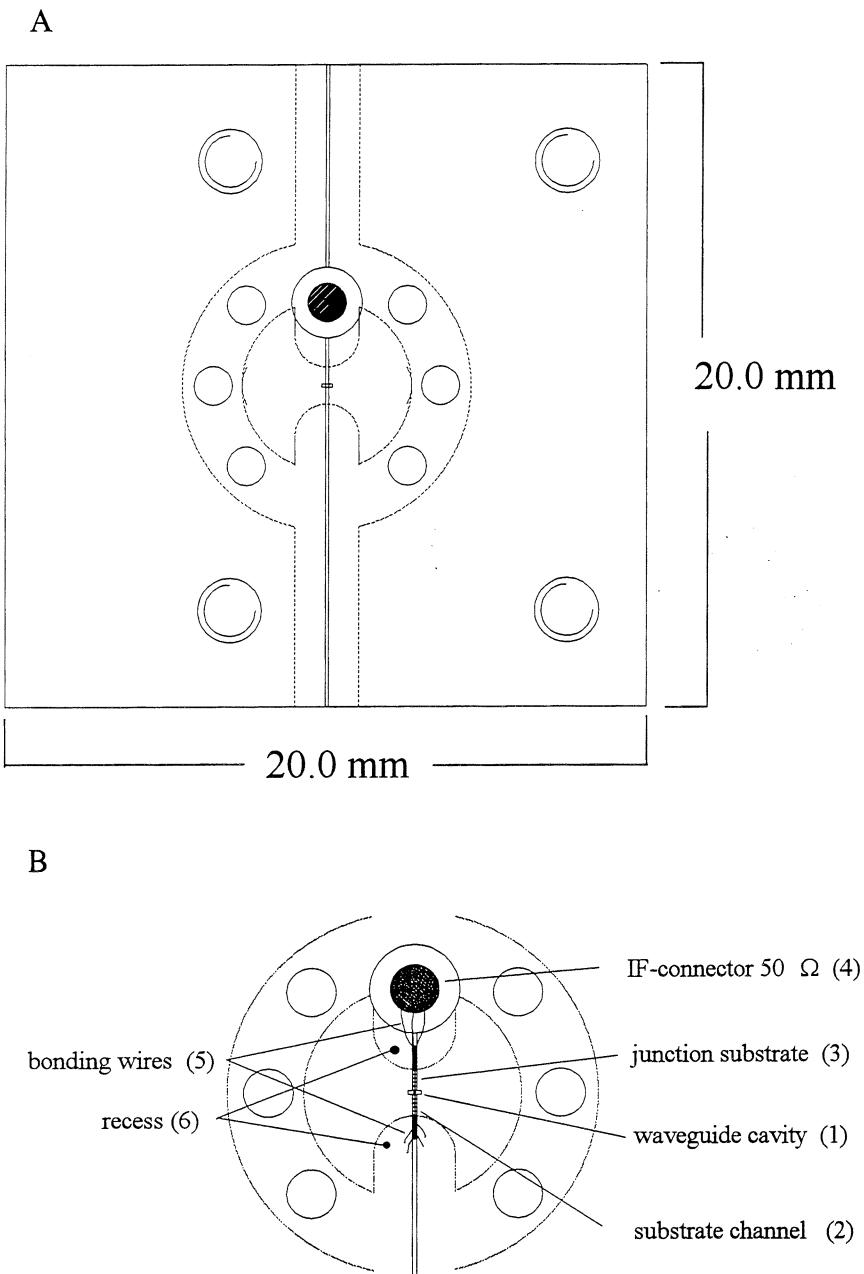
Fig. 2: A) Face-on view of the mixerblock with fixed backshort, B) detail of the central part.
