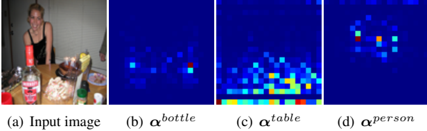
Figure 2. Examples of learned attentions. (a) Input image, (b), (c) and (d) represent attention weights obtained by Eq. (3). The proposed attention model adaptively focuses on different areas in an image depending on input labels.
