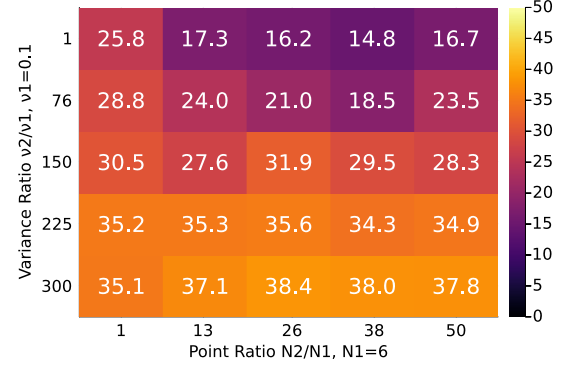
(b) ALPCAUS ( B = 1 , TIPS) mean clustering error.
