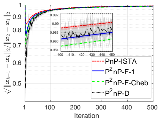
Fig. 8. Numerical test of the convergence rates of PnP-ISTA, P 2 nP-F-1, P 2 nP-F-Cheb, and P 2 nP-D averaged on six brain test images with spiral acquisition. The shaded region of each curve represents the bound of the \rho_k across all brain test images.
