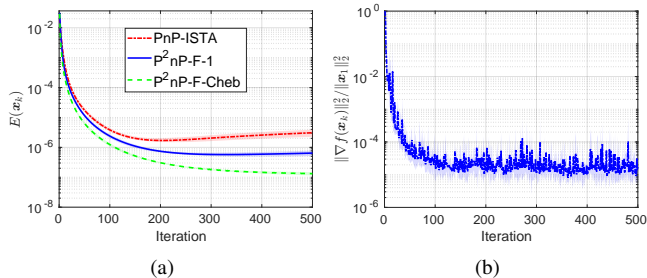
Fig. 7. (a) Numerical test of the fixed-point convergence of PnP-ISTA, P 2 nP-F-1, and P 2 nP-F-Cheb. (b) \|\nabla f(\mathbf{x}_k)\| values versus iteration for P 2 nP-D.
