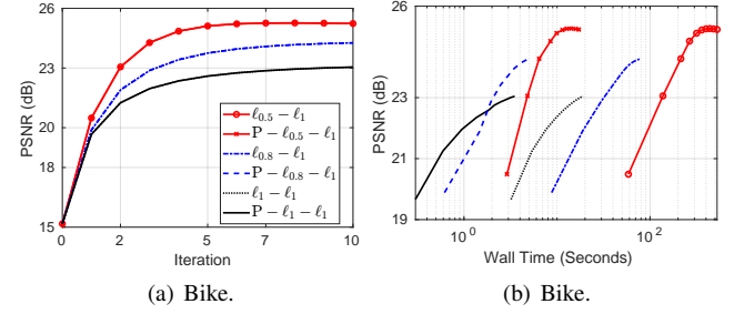
Fig. 4. PSNR values versus iteration and wall time for different p in the image super-resolution task.
