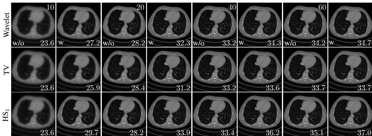
Fig. 8. The parallel-beam CT reconstructed images with wavelet, TV, and HS_1 based regularization at iterations 10, 20, 40, and 60. Columns 1, 3, 5, and 7 (respectively, 2, 4, 6, and 8) show the reconstructions without (respectively, with) RNP. The associated PSNR values are listed at the right corner of each image.
