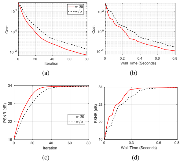
Fig. 10. Comparison of using RNP for TV based CT reconstruction. w/o denotes the one without using RNP.
