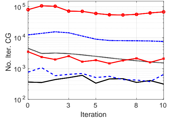
Fig. 5. Number of iterations within CG for different p in the super-resolution task. The downsampling factor is 2. The legend is identical to Figure 4.
