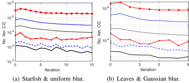
Fig. 3. Number of iterations within CG for different p in the image deblurring task. The legend is identical to Figure 2.
