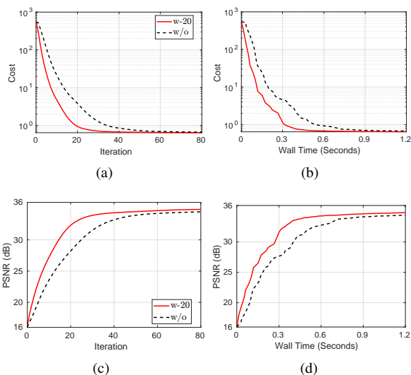
Fig. 9. Comparison of using RNP for wavelet based CT reconstruction. w/o denotes the one without using RNP.
