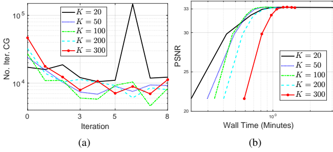
Fig. 6. Comparison of different K in the image deblurring task with Gaussian kernel on the leaves image. (a): the number of iterations within CG in each iteration; (b): PSNR values versus wall time.
