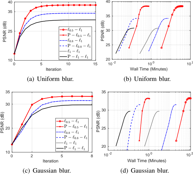
Fig. 2. PSNR values versus iteration and wall time for different p in the image deblurring task. First (respectively, second) row is tested on the starfish (respectively, leaves) image.
