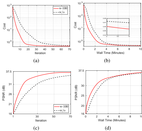
Fig. 11. Comparison of using RNP for HS_1 based CT reconstruction. w/o denotes the one without using RNP.
