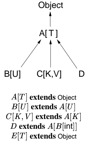
Figure 7: A parameterized class hierarchy
