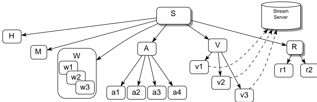
Figure 3. Storage representation of recorded sessions.
