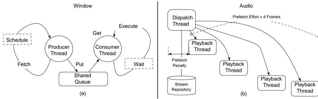
Figure 4. Thread models for replay of the window event stream (a) and for the replay of the continuous audio stream (b).
