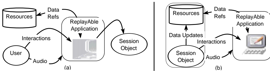
Figure 1. Capture and replay of an interactive session.
