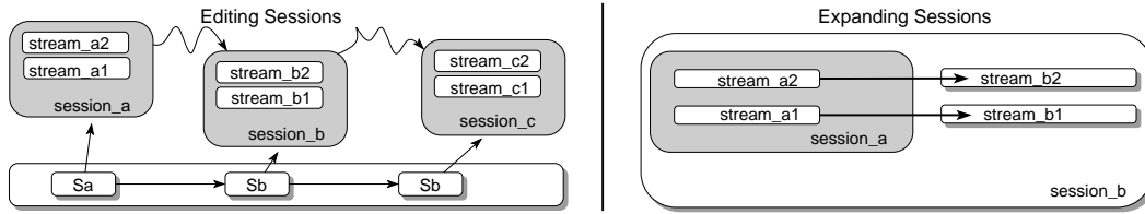
Figure 5. Editing (a) and expanding (b) session objects.
