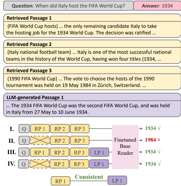
Figure 3: Example for demonstrating the construction of silver consistent labels to train the consistency discriminator \mathcal{D}_C .
