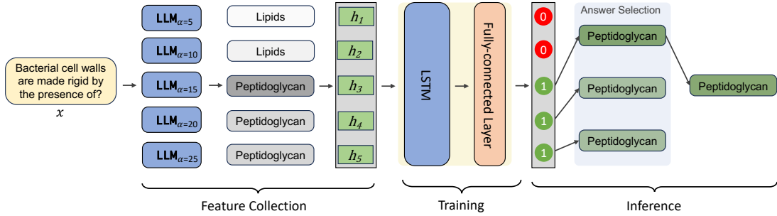
Figure 2: Overview of LITO method. Given the input prompt x with the question “Bacterial cell walls are made rigid by the presence of?”, our method first collects model-generated responses after applying ITI-identified directions at 5 intensities LLM_{\alpha=5k}(x) (Section 3). Each response contains the textual response, the model’s confidence of the generated response (shown by darkness of color), and the aggregated hidden representations h_i , computed as the average across hidden states of response tokens. LITO predicts the accuracy of each response given its hidden representations and selects the accurate response (labeled as 1) with the highest confidence or indicates uncertainty.
