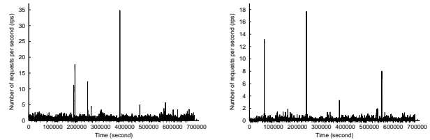
(a) The number of requests per second ( esg )
