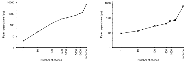
(a) Peak request rate forwarded to the origin (Play-along)
