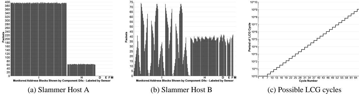
Figure 3. (a, b) Slammer infection attempts from two unique hosts by destination /24s. (c) Period of all possible cycles in the Slammer LCG for b of 0x88215000 .
