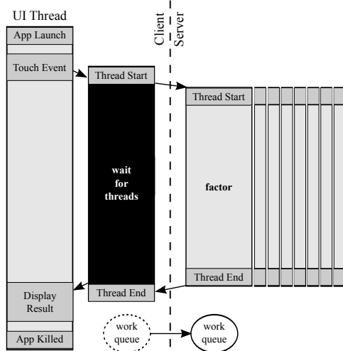
Figure 8: An illustration of multi-threaded execution being offloaded to a server for the Factor application. Time progresses from the top to the bottom of the diagram.
