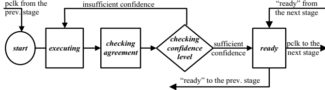
Figure 6. Lockstep synchronization flow.
