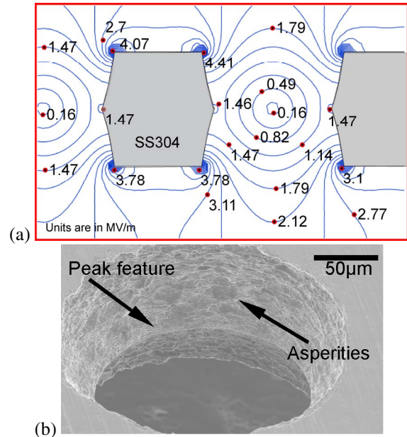
Figure 2: Electric field modeling with V_{\text{applied}} = 600\text{V} (a) A magnified view of the field profile near the perforation feature. Units are in \text{MV/m} . (b) SEM images of the perforations show a top diameter of 225 \mu\text{m} and center diameter of 175 \mu\text{m} .
