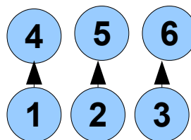
Union-Find Forest
