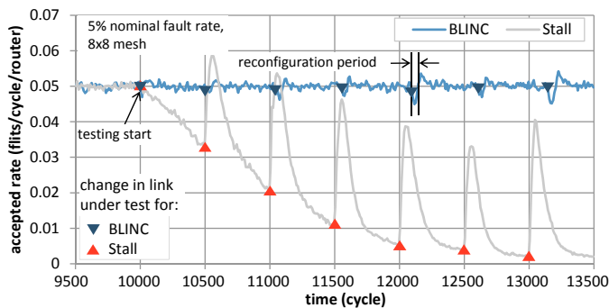
Fig. 9. Accepted flit rate during testing. BLINC shows a steady rate with little fluctuations during reconfiguration (near 12,100 cycle and 13,150 cycle). Stall shows a constantly decreasing rate with periodic peaks.
