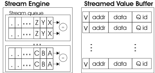
FIGURE 5: Stream engine and streamed value buffer.
