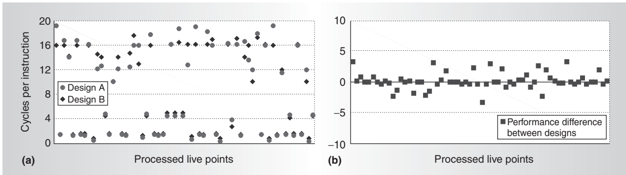
Figure 8. Matched-pair comparison example: performance data for the same sampling unit measured under two microarchitecture designs (a) and performance deltas for each sampling unit (b). The lower variability of performance deltas reduces sample size by 3.5 to 150 times.
