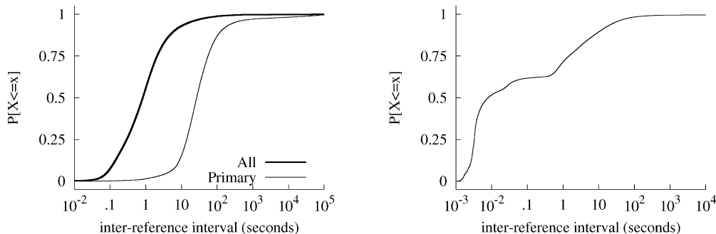
Fig. 8. Distribution of inter-reference intervals in WebTV (left) and Boston University (right) client traces.
