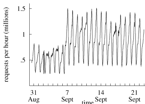
Fig. 2. Hourly request volume.
