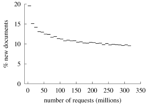
Fig. 5. Percentage of replies containing new documents.
