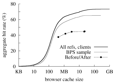
Fig. 10. Aggregate WebTV client success function.
