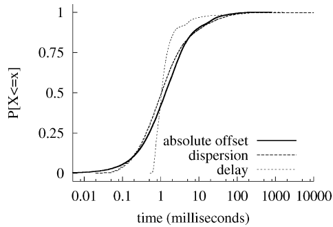
Fig. 1. Distribution of NTP parameters during data collection.
