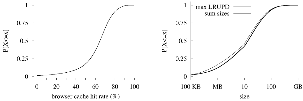
Fig. 9. Distribution of maximal browser hit rates (left) and effectively infinite browser cache sizes (right).
