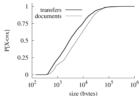
Fig. 4. Distribution of document and transfer sizes.
