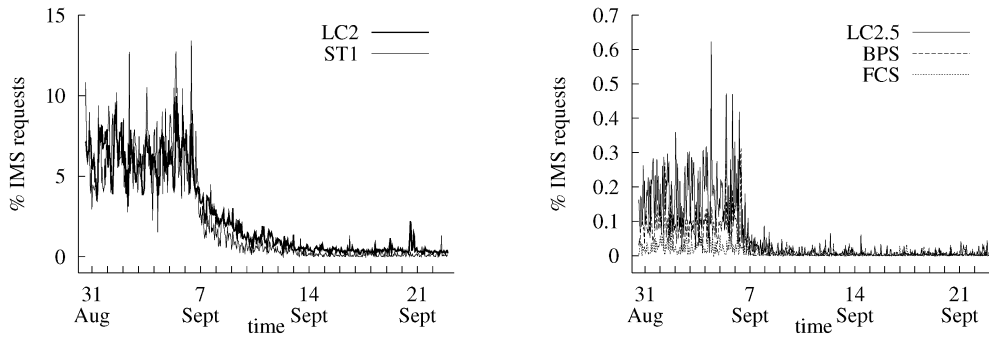
Fig. 3. Percentage of IMS requests from diskful (left) and diskless (right) clients, 1-h bins. Vertical scales differ.
