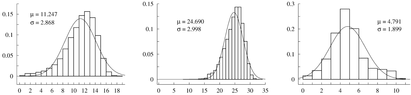
Fig. 7. Histograms of log 2 -transformed data: left: references/client. Center: bytes/client. Right: stack distances in BPS sample.
