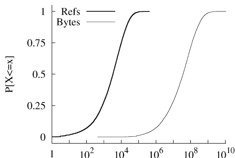
Fig. 6. Distribution of references/client and bytes/client.
