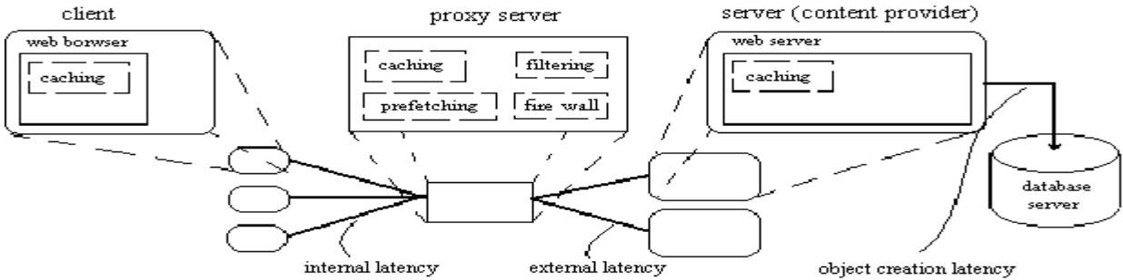
Figure 1 - General WWW Architecture
