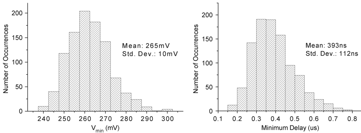
Fig. 8. (a) Simulated distribution of V_{\min} for a chain of 30 inverters subject to gate length and V_{th} variations. (b) Distribution of minimum delay, t_{\min} , for the same inverter chain with V_{dd} fixed at 265 mV.
