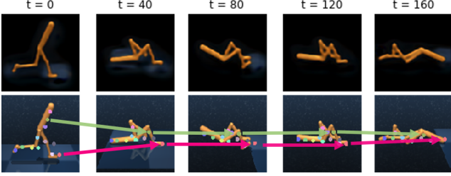
Figure 4: Our VAI foreground reconstruction (Row 1) provides clearer and more robust foreground visual information than detecting keypoints across image frames using Transporter (Row 2). Due to occlusion, symmetry, and lacking visual distinctions, it is often impossible to track keypoints consistently across frames. That is, keypoint locations alone are not suitable as an invariant visual representation.
