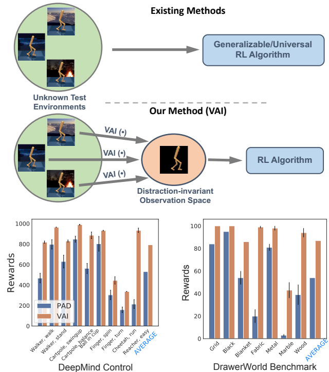
Figure 1: Top ) Two ways to make vision-based reinforcement learning generalizable to unknown environments at the test time: Existing methods focus on learning an RL policy that is universal to varying domains, whereas our proposed Visual Attention and Invariance (VAI) extracts visual foreground that is universal, feeding clean and invariant vision to RL. Bottom ) VAI significantly outperforms PAD (SOTA), increasing cumulative rewards by 49% and 61% respectively in random color tests on DeepMind control and random texture tests on our DrawWorld manipulation benchmarks.
