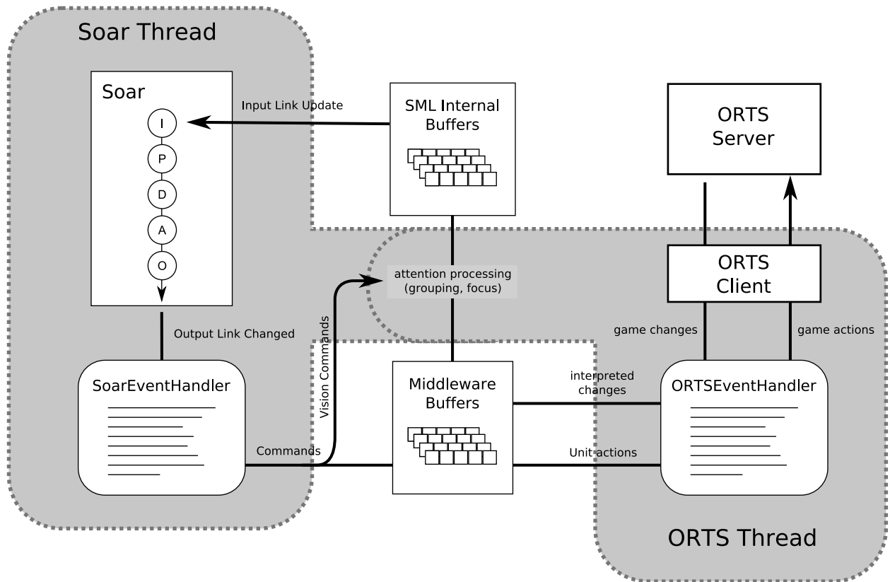
Figure 3: Overview of how control is passed through Sorts. Note that the two gray regions represent two different threads executing asynchronously.
