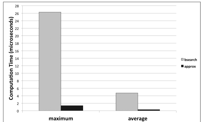
Figure 3. Synthetic prediction approximation efficiency evaluation.
