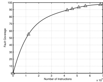
Fig. 2: Fault coverage achieved (in percentage) for varying number of software based self test instructions.
