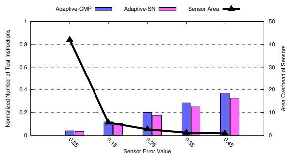
Fig. 7: Number of test instructions for the adaptive online testing in CMP and SN with varying amount of sensor error. The number of test instructions are normalized to a regular CMP with fixed periodic testing. The plot also shows the sensor area overhead used by the proposed approach for health assessment. The coverage target ( SC ) is fixed at 97.3%.
