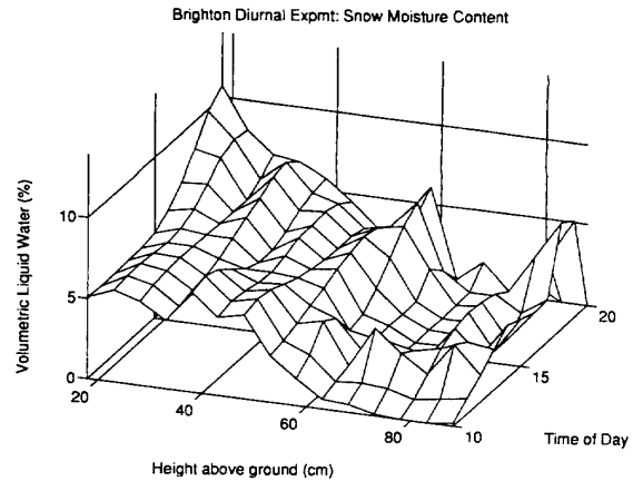
Fig. 12. Snow moisture measured via the snow probe in a 0.88-m snowpack over a diurnal cycle, shown as a function of time and height above the ground.
