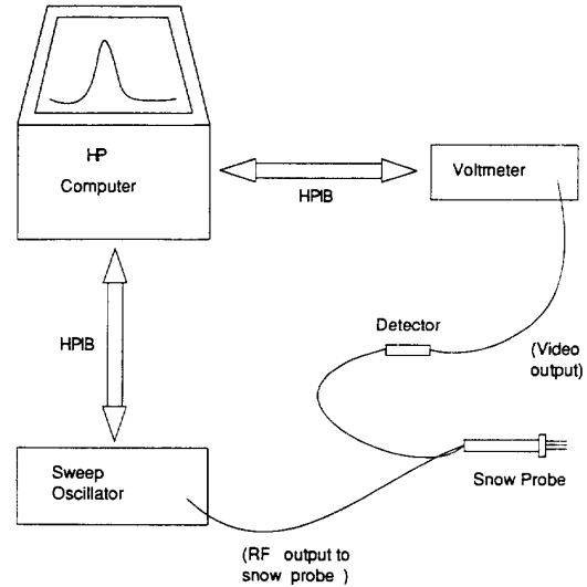
Fig. 2. Schematic diagram of snow probe system.
