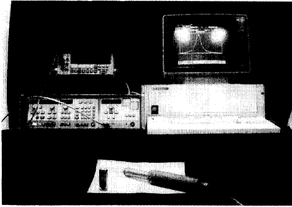
Fig. 1. Photograph of snow probe system.
