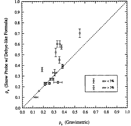
Fig. 7. Comparison of snow density results obtained via snow probe (in conjunction with Debye-like relation) and gravimetric measurements. Data points represented with squares were from snowpacks having volumetric wetness levels of >3\% ; with circles, <3\% .
