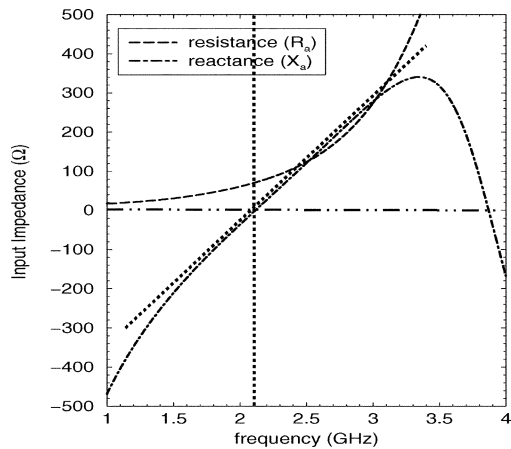
Fig. 5. Input impedance of dipole antenna in free space.
