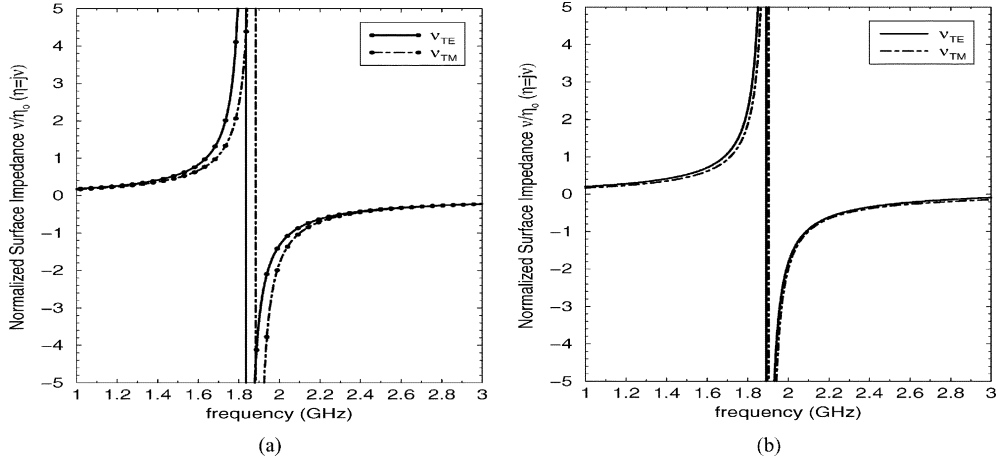
Fig. 13. Oblique incident surface impedance performance of the RIS substrate for arbitrary plane wave \theta^i = 90^\circ , \theta^r = 120^\circ , \psi^i = 50^\circ [coordinate system is defined in Fig. 9(a)]. (a) Circuit model approach and (b) FDTD technique. Comparing to Fig. 12, the surface reactance is almost independent of polarization and incidence angle.
