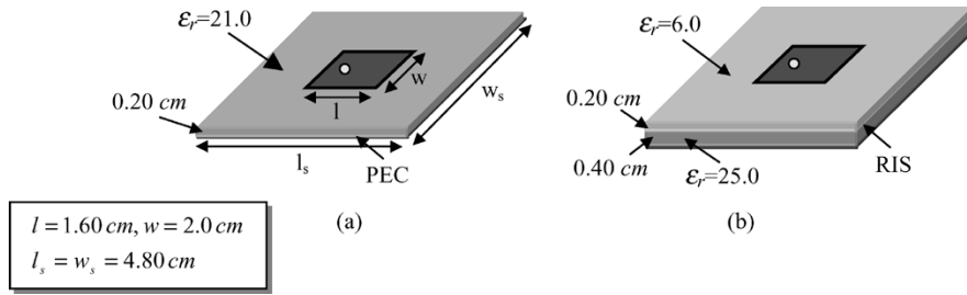
Fig. 18. Patch antenna on the (a) conventional substrate and (b) RIS substrate (a 4 × 4 array of square patches printed on the PEC-backed dielectric material).
