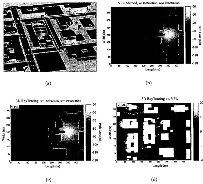
Fig. 2. Comparison of the quasi-3D VPL method with full 3D ray tracing for downtown Ann Arbor, Michigan. (a) Rendition of Ann Arbor, Michigan, (b) VPL results, (c) 3D results, (d) VPL path loss minus 3D path loss.
