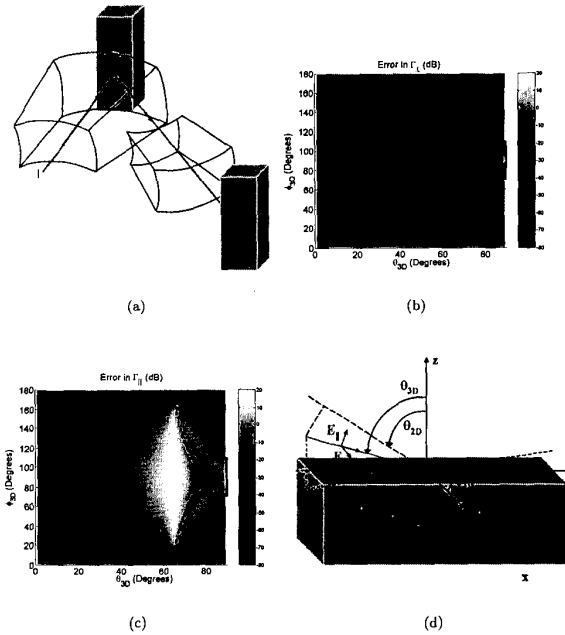
Fig. 1. Intelligent ray tracing (a) , Error in Fresnel Reflection Coefficients for 2D approximation, (b) Perpendicular Polarization, (c) Parallel Polarization, (d) problem geometry.
