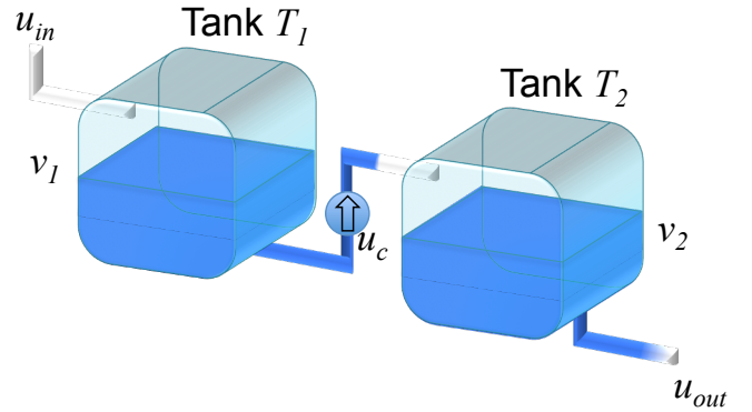
Fig. 1. Fuel tank system.
