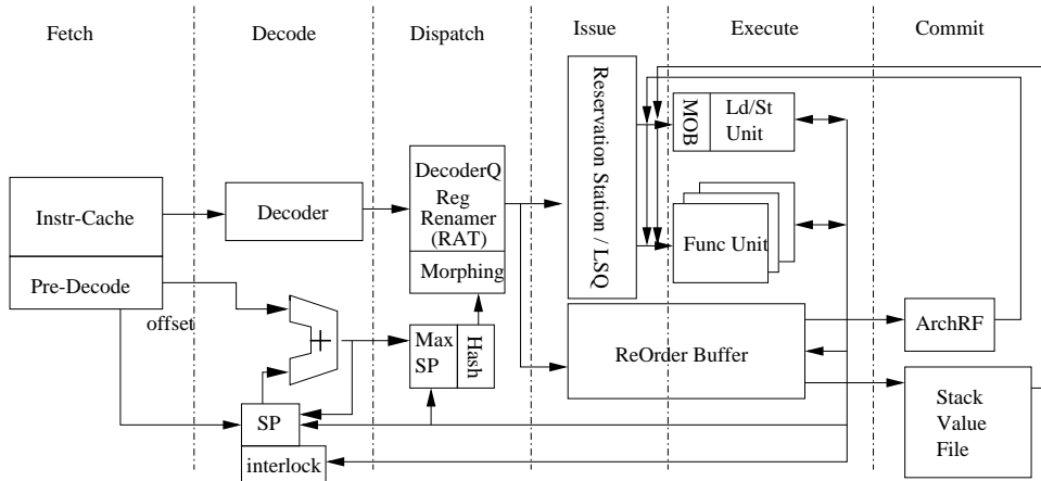
Figure 4: Microarchitecture Extension with a Stack Value File Implementation
