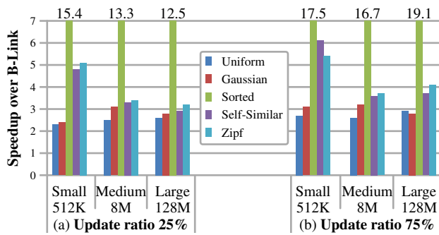
Figure 6: Relative performance of PALM as compared to B-link Trees for small, medium and large trees of 4-byte keys on different distributions and update ratios of (a) 25% and (b) 75%. PALM is 2.3X – 19.1X faster than B-link Trees.
