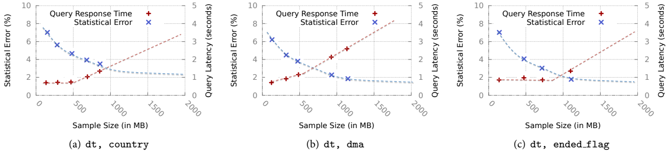
Figure 6. Error Latency Profiles for a variety of samples when executing a query to calculate average session time in Galena. (a) Shows the ELP for a sample biased on date and country, (b) is the ELP for a sample biased on date and designated media area (dma), and (c) is the ELP for a sample biased on date and the ended_flag.
