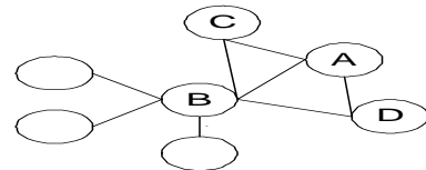
Figure 12: Correlated Attacks.
