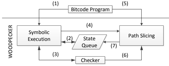
Figure 3: WOODPECKER architecture.
