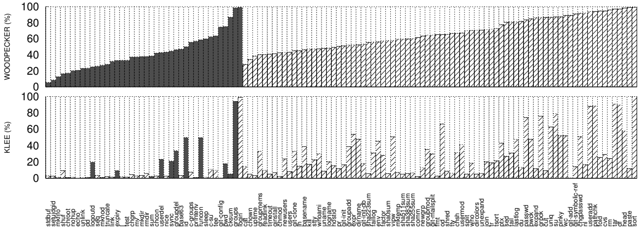
Figure 9: Search efficiency with the file access checker. WOODPECKER's median search efficiency of the hatched bars is 65.4%, whereas KLEE's is 20.9%.
