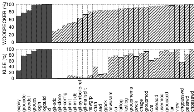
Figure 10: Search efficiency with the data loss checker. WOODPECKER's median search efficiency of the hatched bars is 89.4%; KLEE's is 71.1%.
