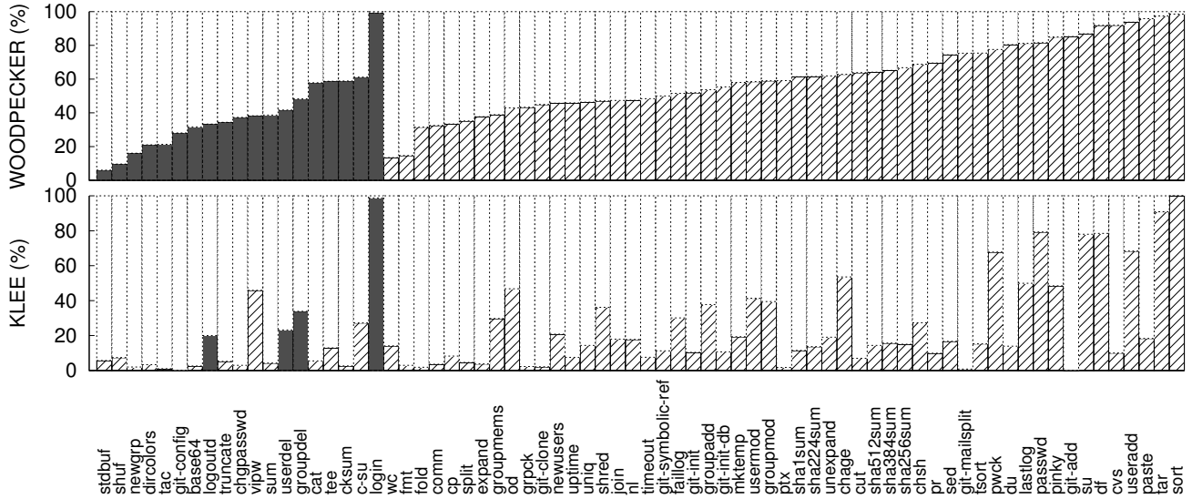
Figure 8: Search efficiency with the open-close checker. WOODPECKER's median search efficiency of the hatched bars is 59.2%, whereas KLEE's is 15.3%.
