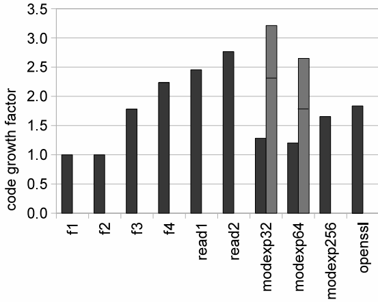
Fig. 3. Code size increase after applying if-conversion and elimination of variable latency division instructions
