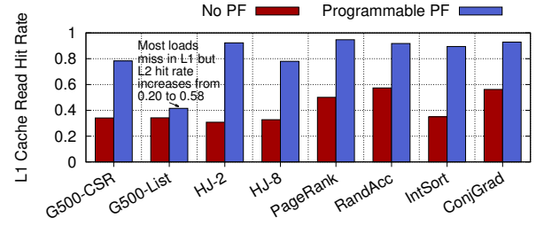
(b) L1 read hit rate
